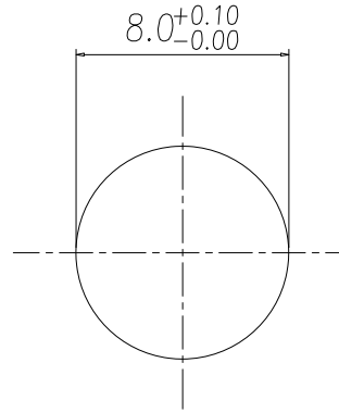
RECOMMEND PANEL CUT-OUT
