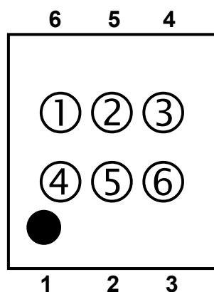
DFN(PL)7/25/2024-6-GZ Marking
