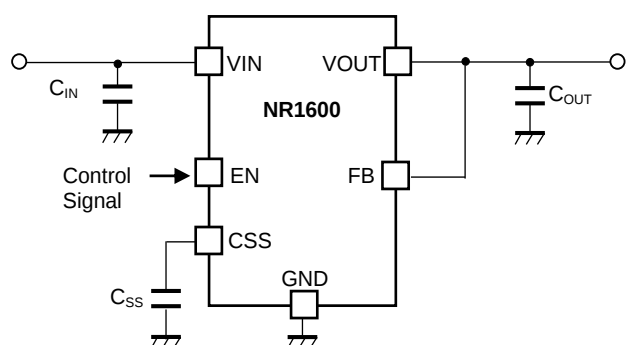
NR1600xxxxxA/D (Fixed Output Voltage Type)
