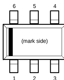
NR1600DD (SOT-23-6-DD) Pin Configuration
