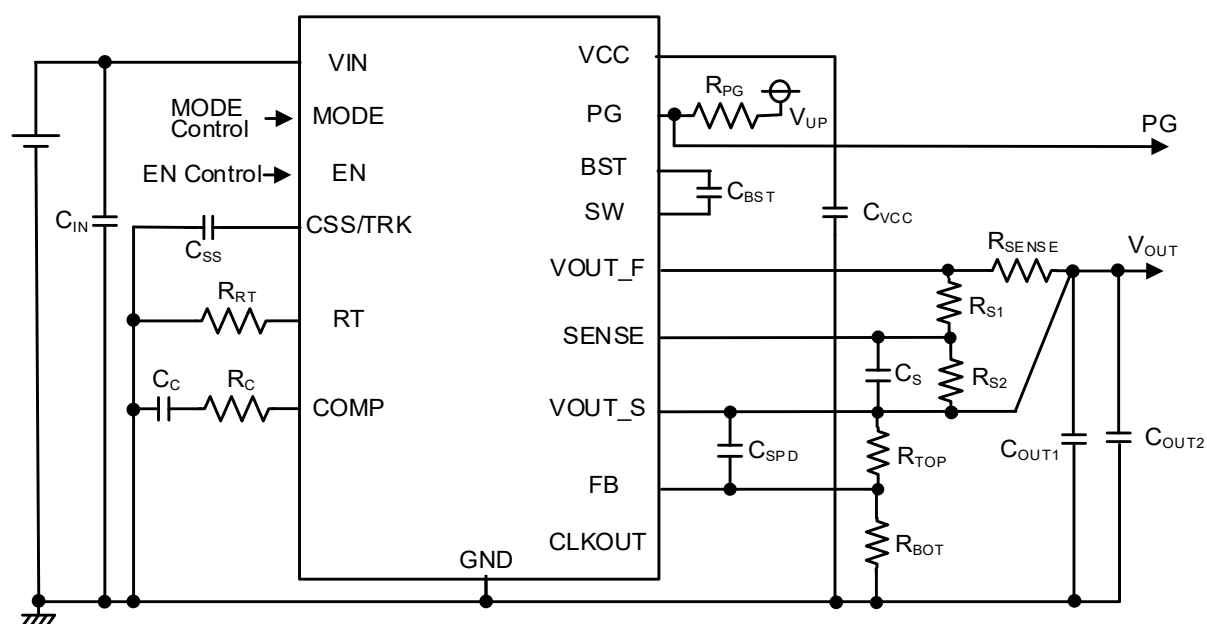
NC2701MA Test Circuit
