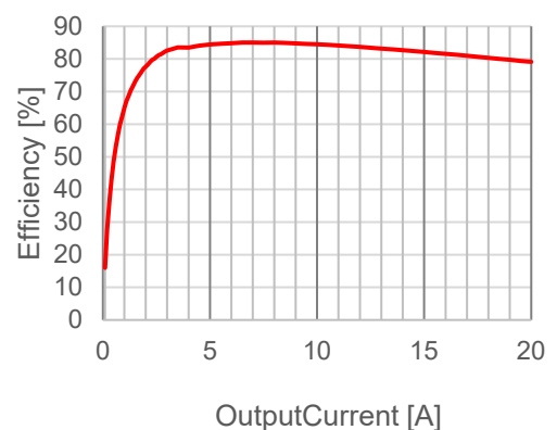
NC2700MA Efficiency Characteristics V IN =12V V OUT =1V F osc =400kHz
