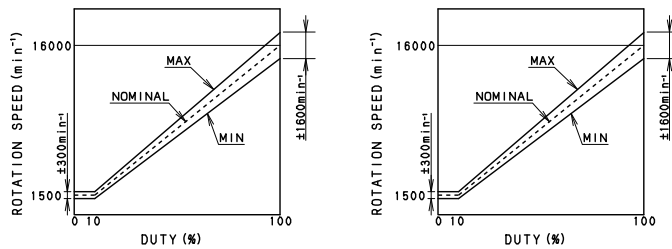
Detail of PWM curve(Inlet side)
