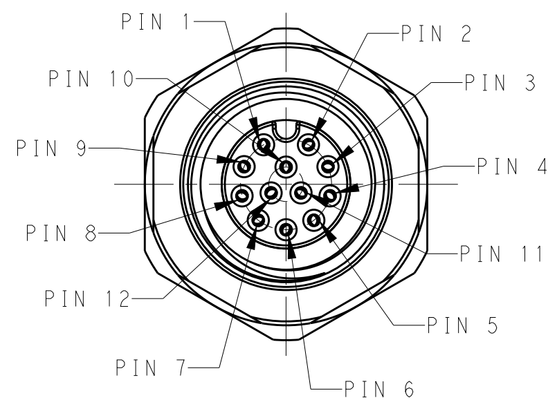
M12, FEMALE, 12POLES
