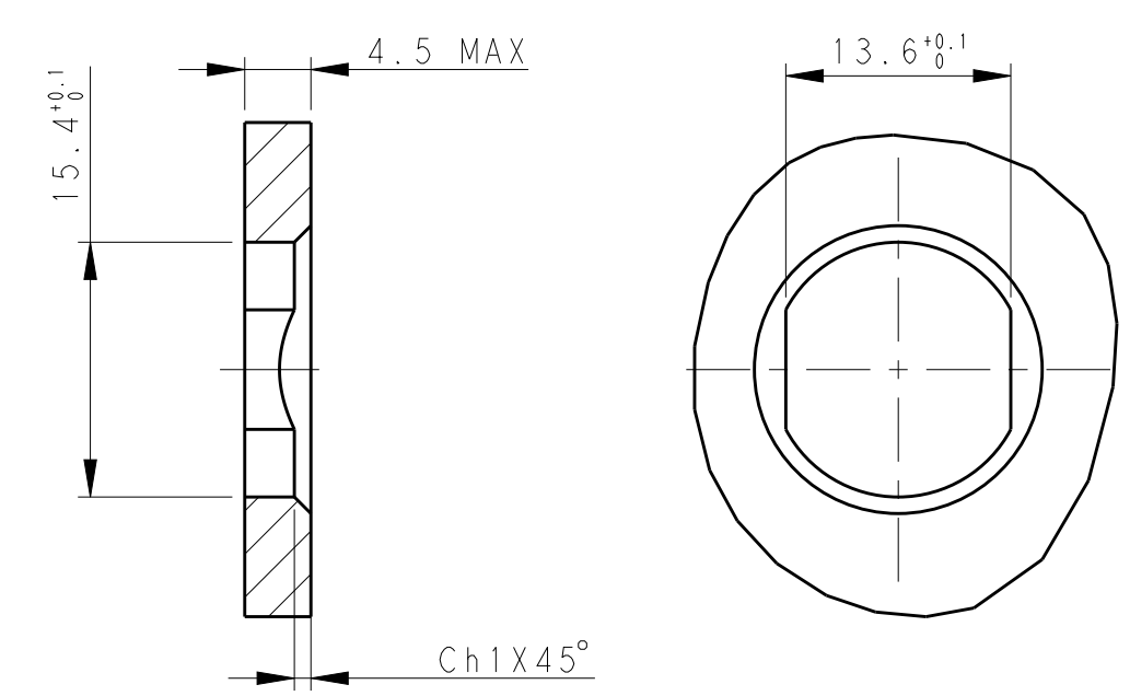
RECOMMENDED PANEL CUTOUT
