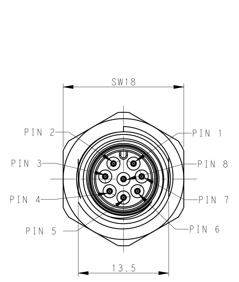
M12, MALE, 8POLES
