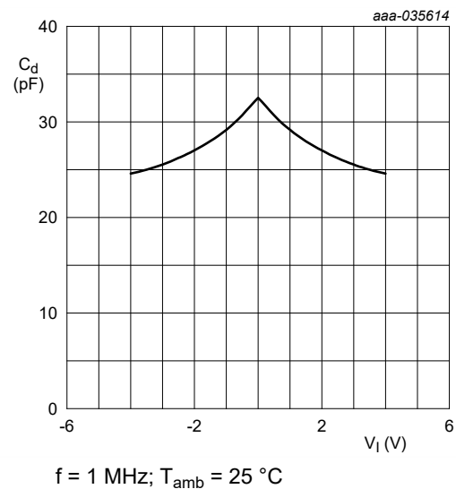
Fig. 4. Diode capacitance as a function of input voltage; typical values
