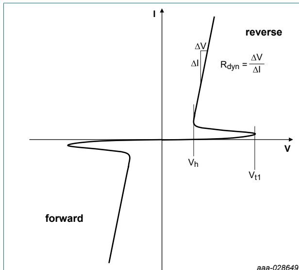
Fig. 3. Definition of snap-back voltage and trigger voltage in a Transmission Line Pulse (TLP) diagram
