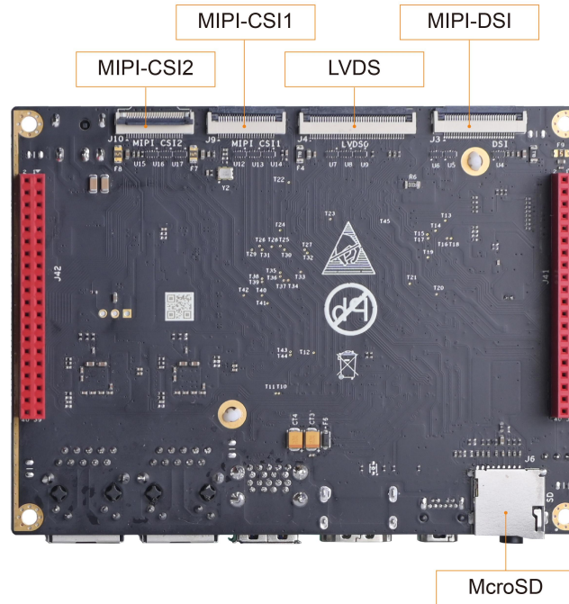
MYD-LT527 Development Board Bottom-view
