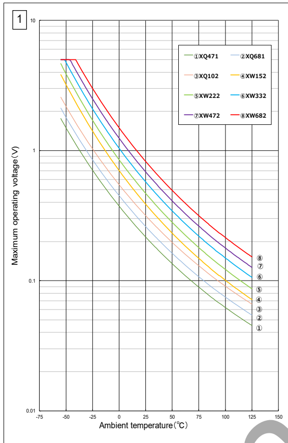
Graph of Maximum Operating Voltage Reduction Characteristics
