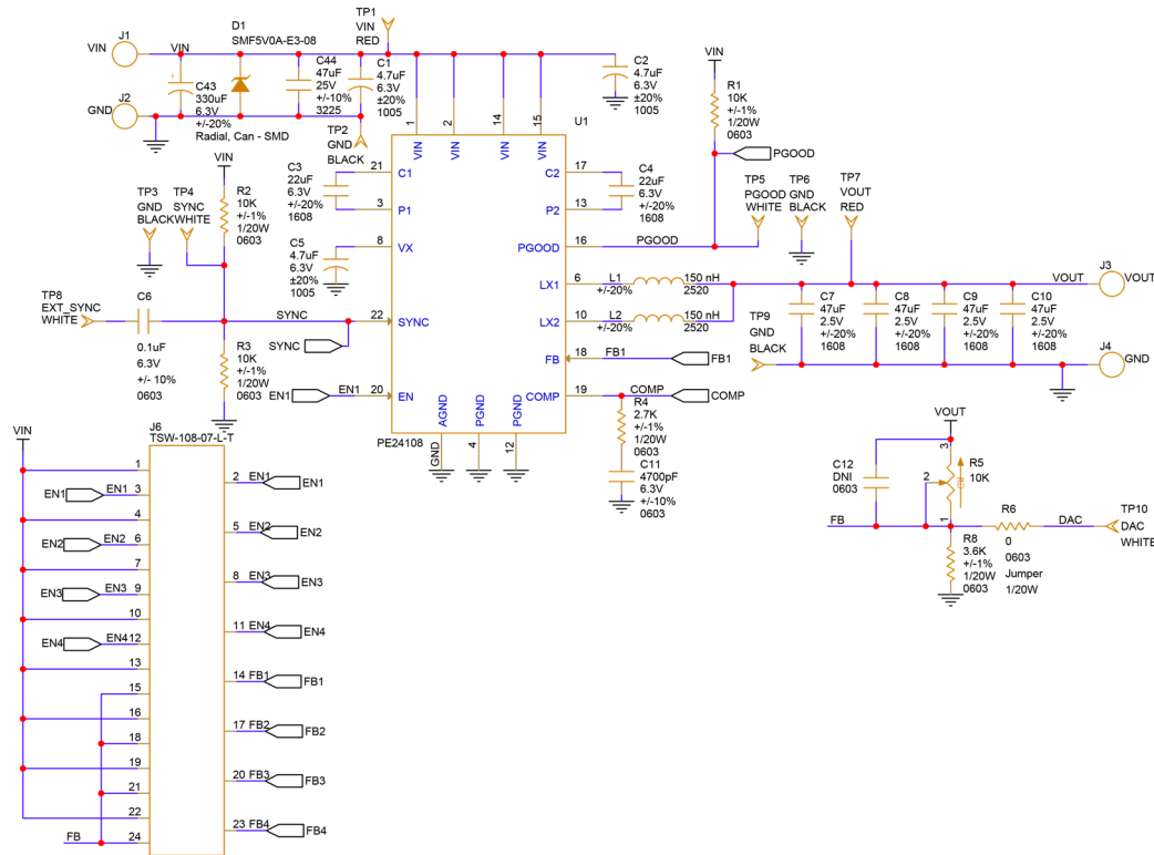
Figure 13. Evaluation Board Schematic, U1 Circuit
