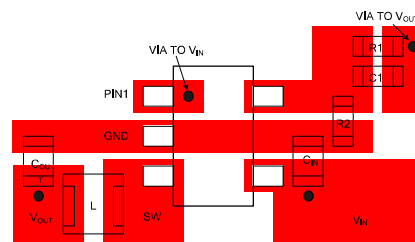
Figure 3. RT8059GJ5-MS Suggested Layout
