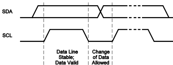
Figure 7. Bit Transfer on the I 2 C Bus
