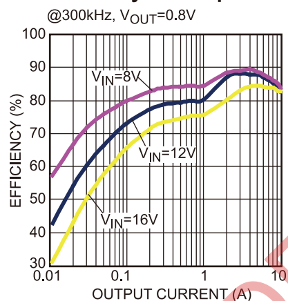
Figure 22 — Efficiency Curve
