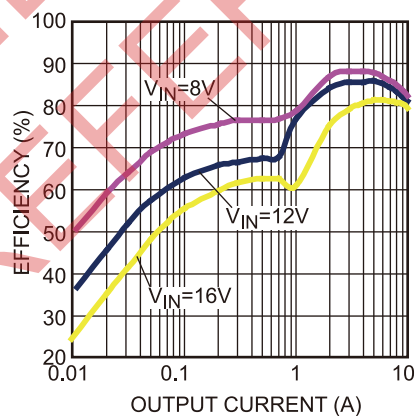
Figure 24 — Efficiency Curve
