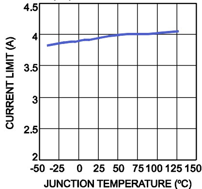
DC Converter Current Limit vs. Temperature Duty Cycle = 35%
