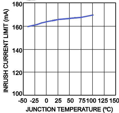
PD Inrush Current Limit vs. Temperature R_{ILIM} = 178k\Omega
