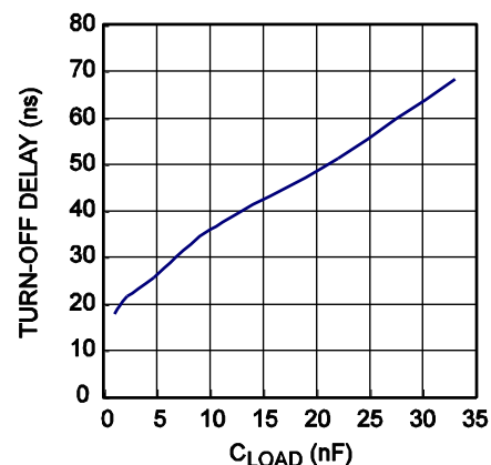
Figure 10: Turn-Off Delay vs. C_{LOAD}
