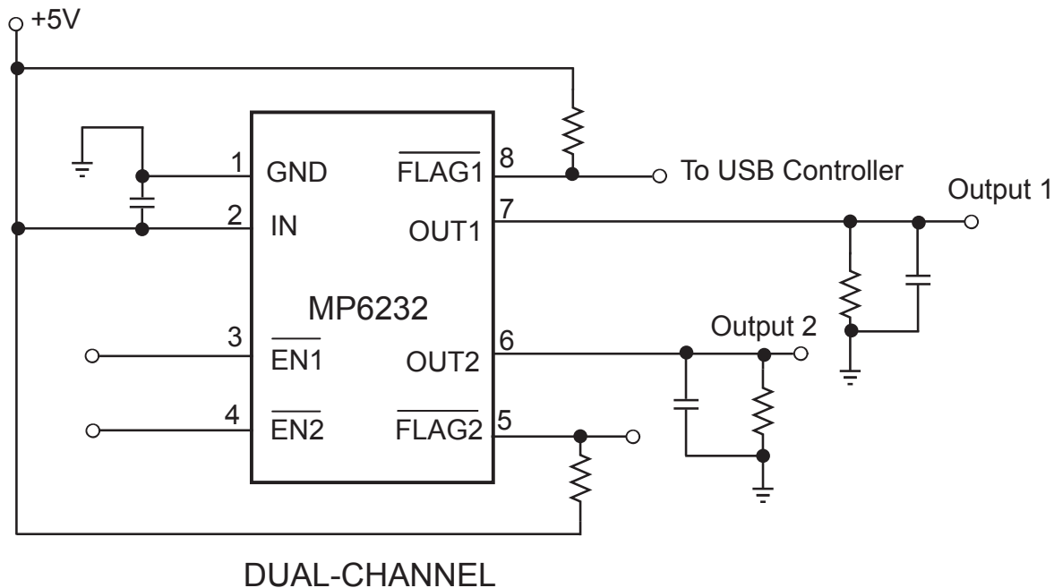
Figure 3—Application Circuit
