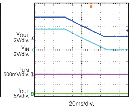
Power Down
