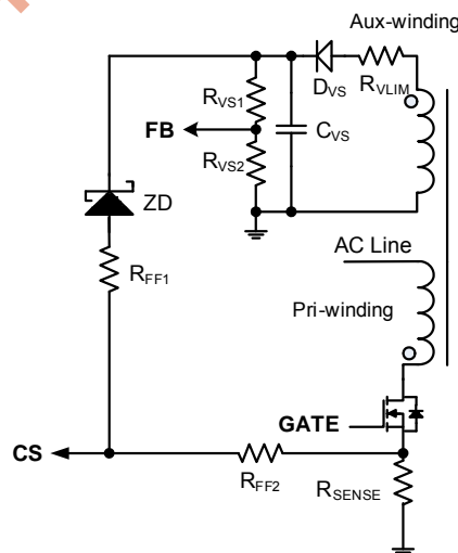
Figure 14—The Feedforward Compensation on CS Pin
