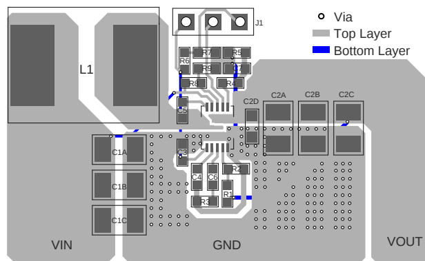
Figure 5: Layout Recommendation
