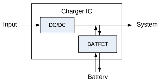
Figure 4: NVDC Power Path Management Structure
