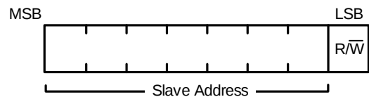
Figure 13: 7-Bit Address
