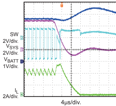
SYS Short Circuit Entry
