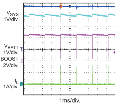
SYS Over Voltage Protection
