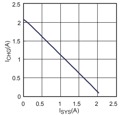
Current Sharing
