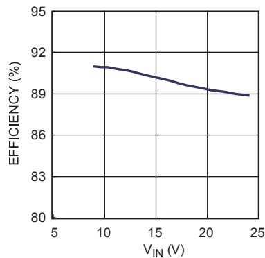
Efficiency vs. V IN 2-Cell, V BATT =7.4V, CC Load
