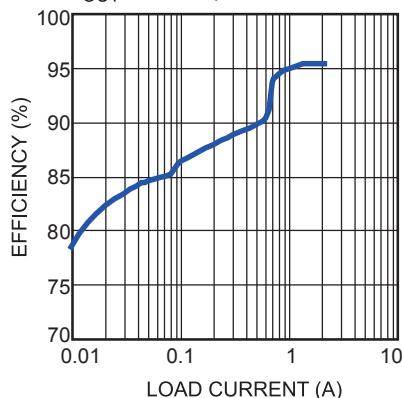
Efficiency vs. Output Current V_{OUT}=5V , L=10\mu H
