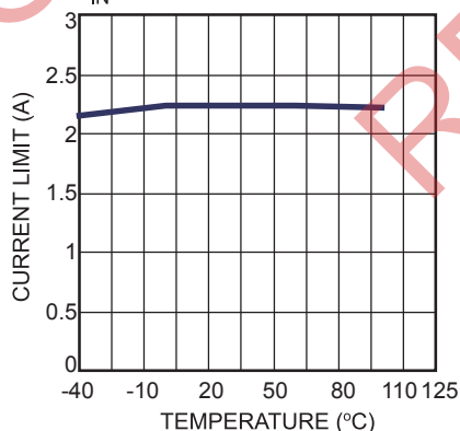
Current Limit vs. Temperature V_{IN}=19V
