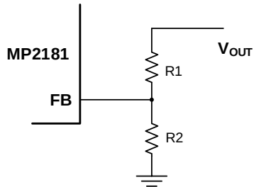
Figure 7: Feedback Network
