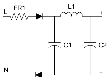
Figure 9: Half-Wave Rectifier
