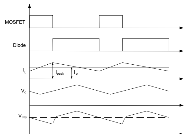
Figure 3: Constant-Voltage Regulation
