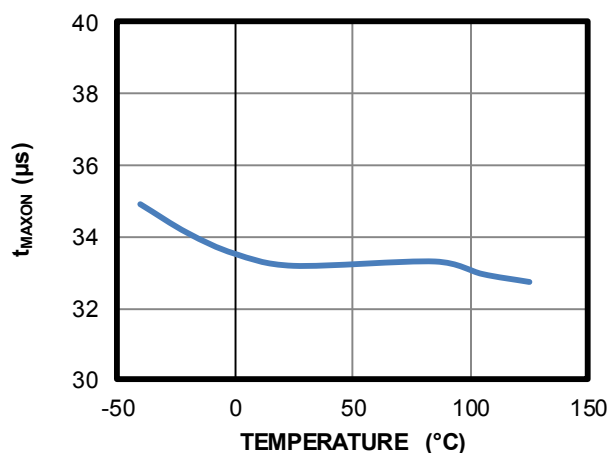
Open-Loop Detection vs. Temperature
