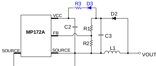
Figure 7: Auxiliary VCC Supply Circuit
