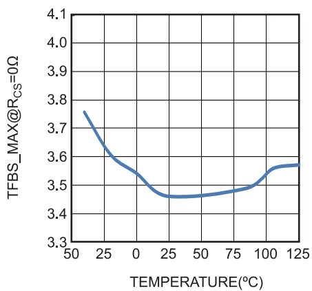
TFBS\_MAX@R_{CS}=0\Omega vs. Temperature
