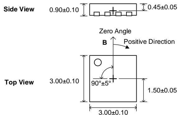
Figure 4: Detection Point and Default Positive Direction
