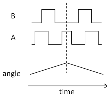
Figure B1: Mechanical Angle Changing from CW to CCW Direction at Dotted Line
