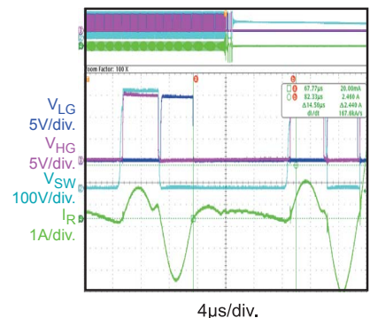
Capacitive-Mode Protection
