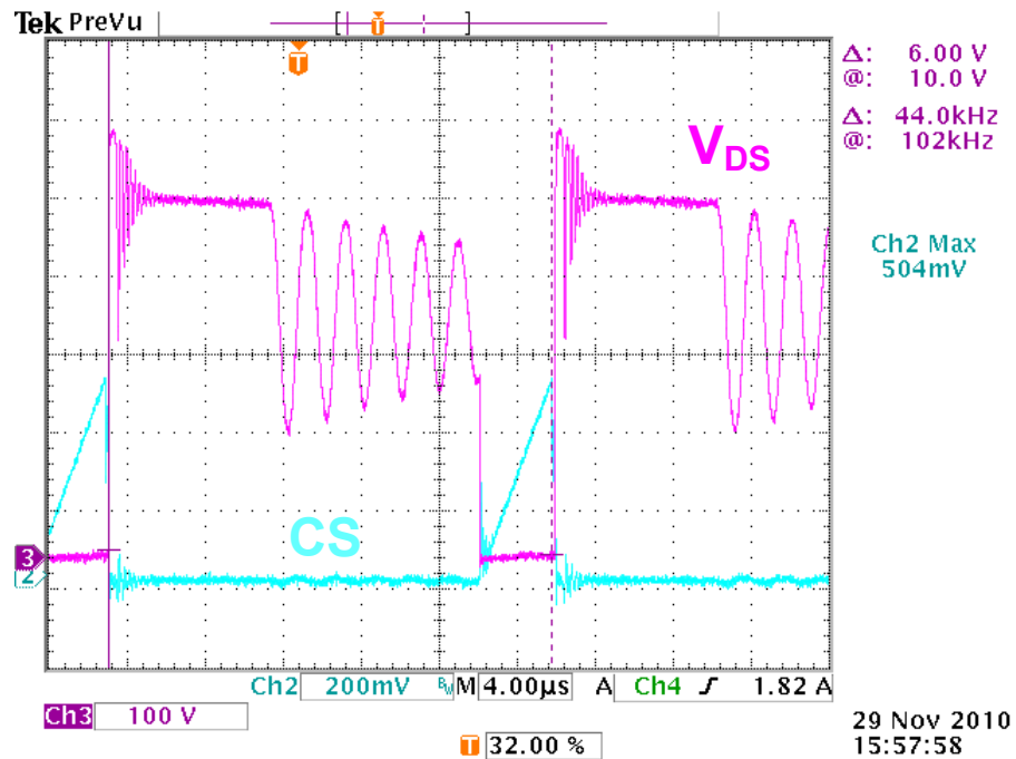
Figure 18: Drain Current and Voltage of MOSFET at High-Line Input (230VAC); CH2 - V_{DS} , CH3, I_D
