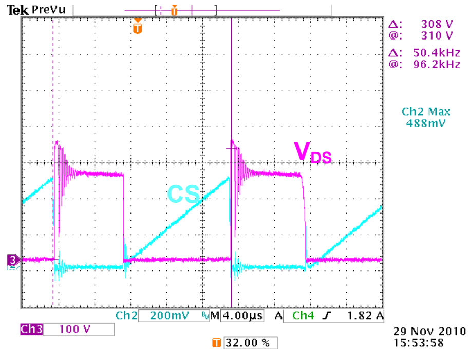
Figure 17: Drain Current and Voltage of MOSFET at Low-Line Input (90VAC); CH2 - V_{DS} , CH3, I_D
