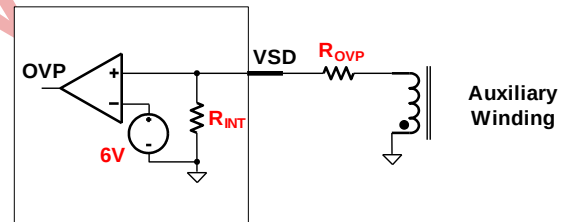
Figure 8—OVP Circuit
