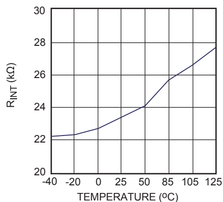
VSD Internal Impedance Level vs. Temperature
