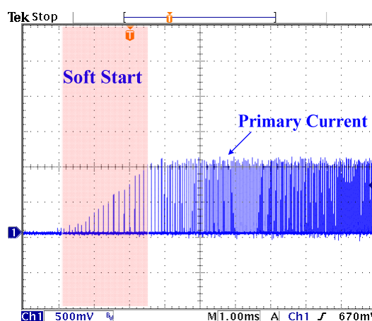
Figure 4—Soft Start
