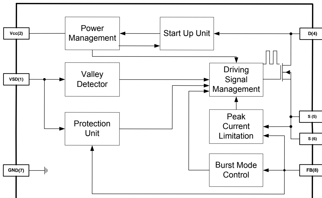
Figure 2—Block Diagram
