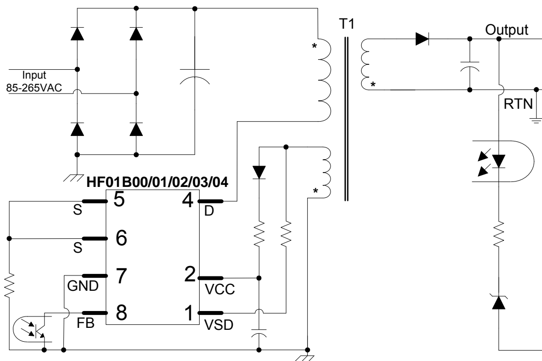
Figure 1—Typical Application
