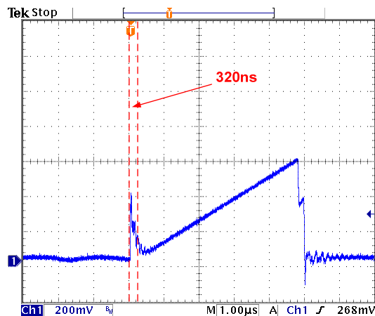
Figure 11—Leading Edge Blanking
