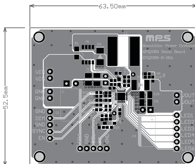
Figure 1: Top Layer
