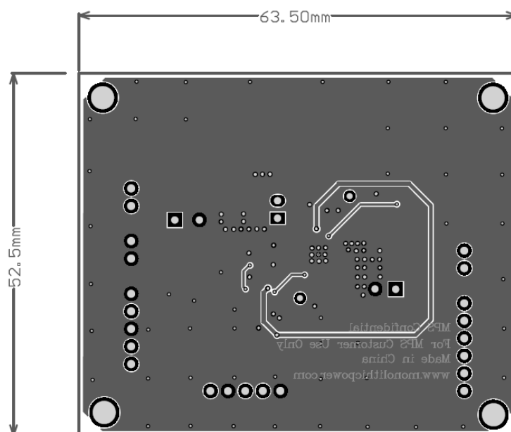
Figure 2: Bottom Layer
