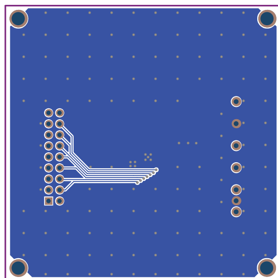
Figure 4: Bottom Layer
