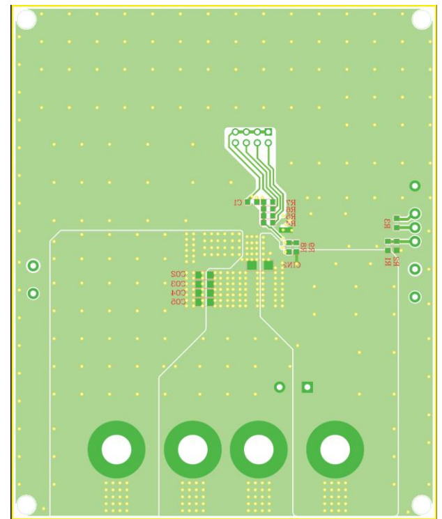
Figure 4: Bottom Layer
