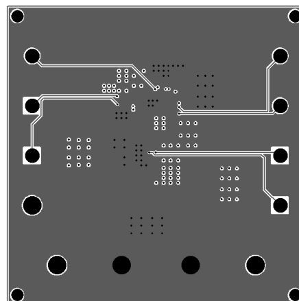
Figure 4: Inner Layer 1
