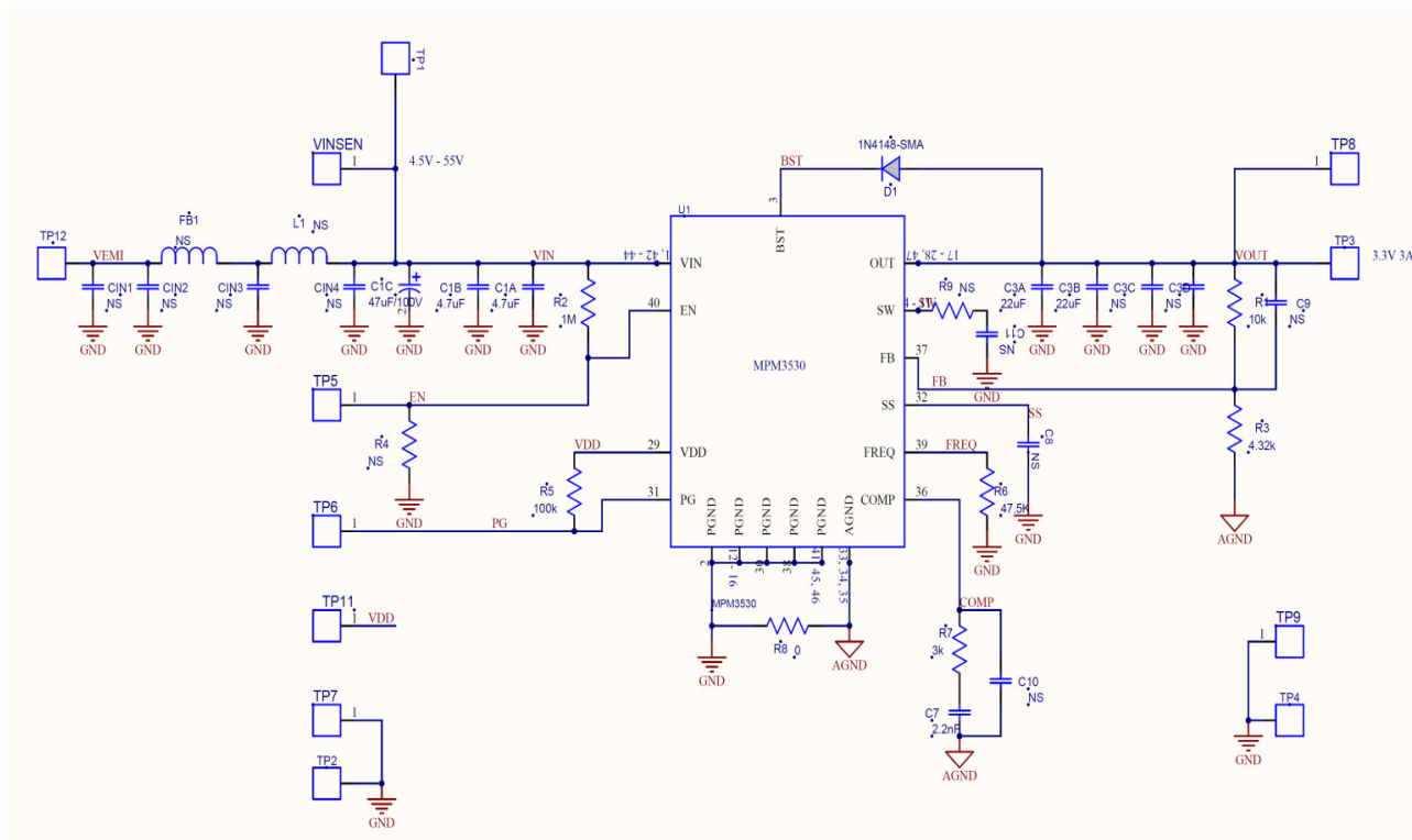
Schematic: V_{in} = 4.5 - 55V , V_{out} = 3.3V
