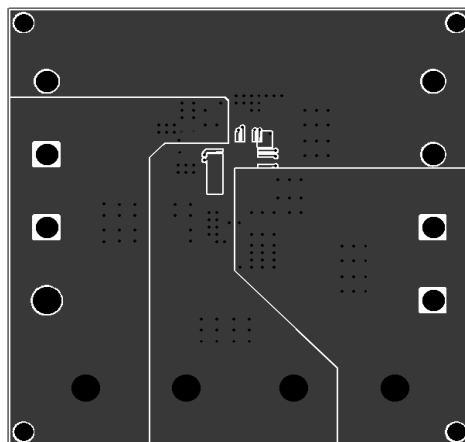
Figure 2: Top Layer
