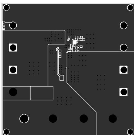
Figure 3: Bottom Layer
