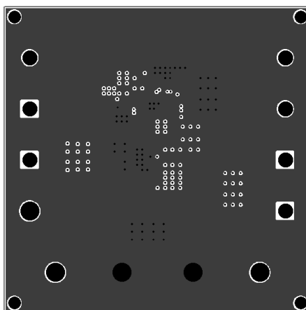
Figure 5: Inner Layer 2
