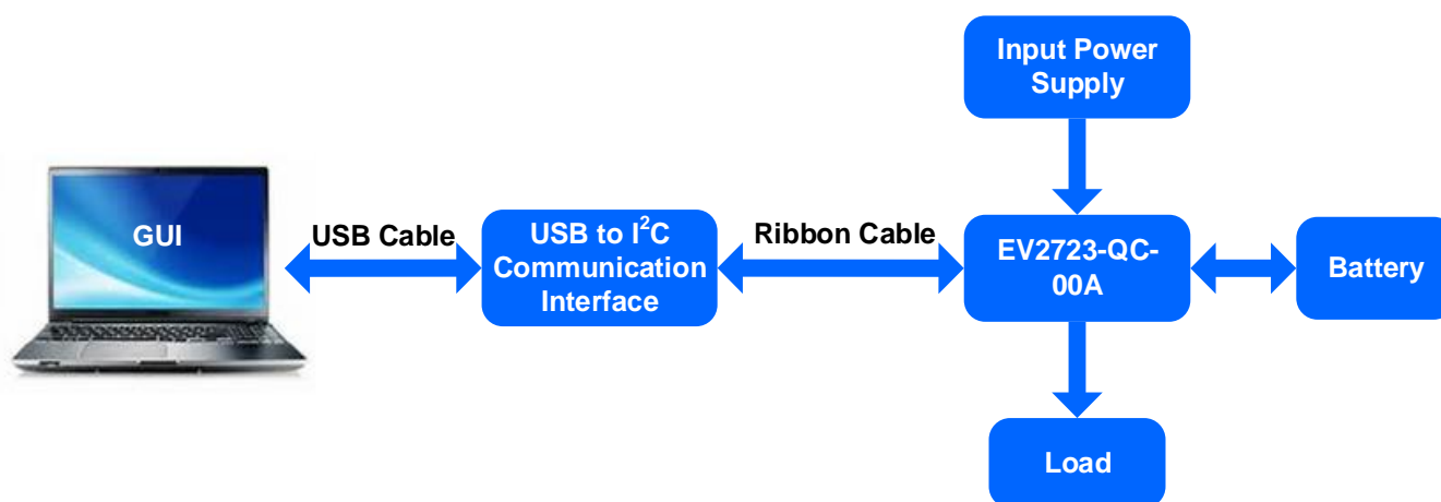
Figure 1: EVKT-MP2723 Evaluation Kit Set-Up
