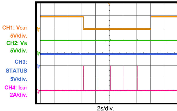
Short-Circuit Protection Entry and Recovery
