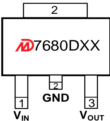
TO252-2L(D_Type) TOP View
