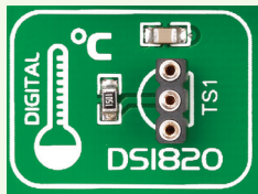
Figure 20-1: DS1820 socket
