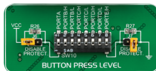
Figure 6-5: Button press level DIP switch (tri-state)
