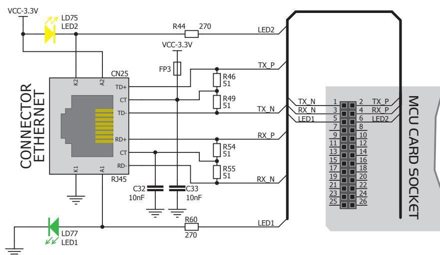
Figure 12-1: Ethernet connection schematic
