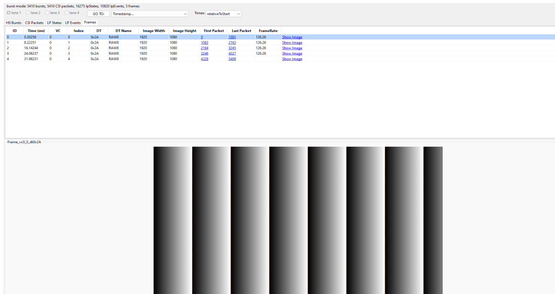
Figure 4-14. Test Pattern—MIPI Analyzer
