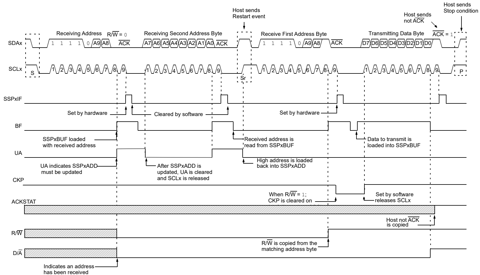
FIGURE 15-22: I 2 C CLIENT, 10-BIT ADDRESS, TRANSMISSION (SEN = 0, AHEN = 0, DHEN = 0)
