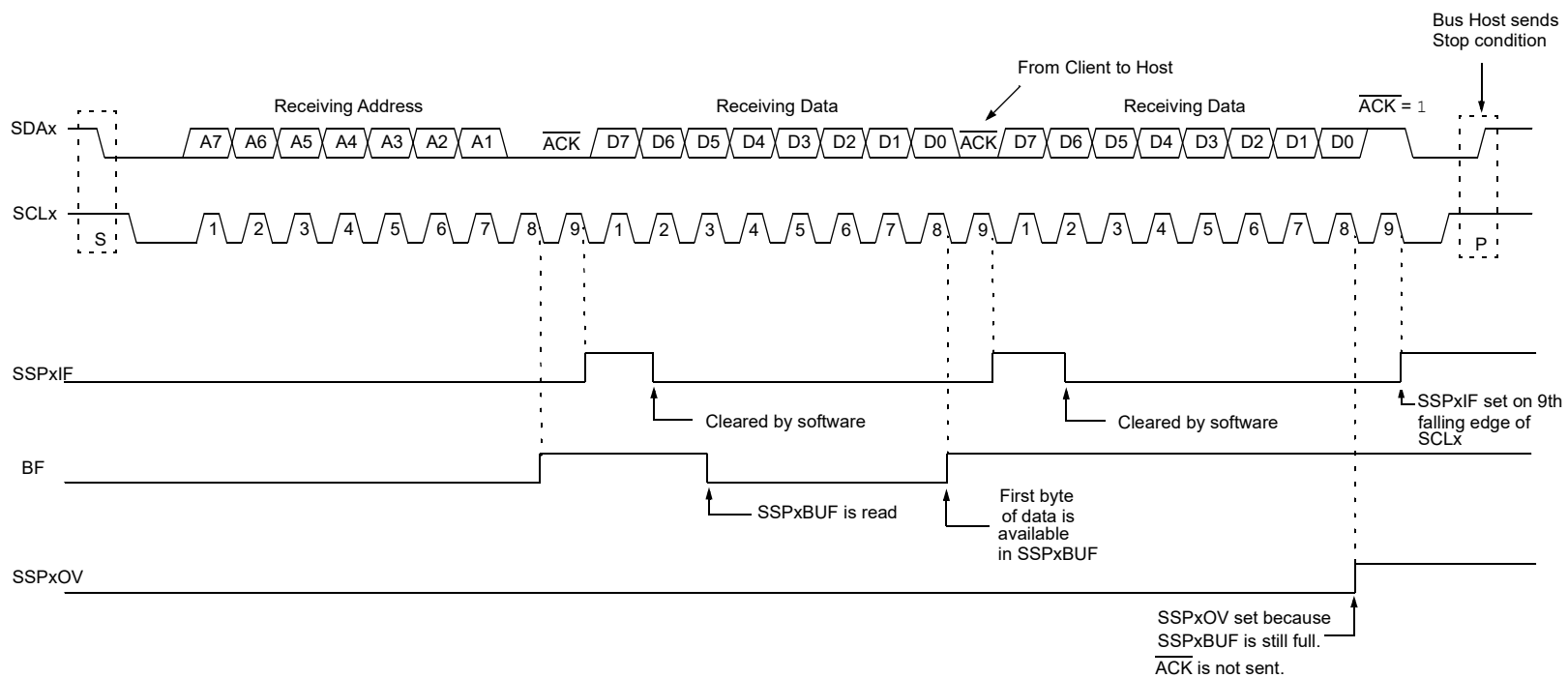
FIGURE 15-14: I 2 C CLIENT, 7-BIT ADDRESS, RECEPTION (SEN = 0, AHEN = 0, DHEN = 0)
