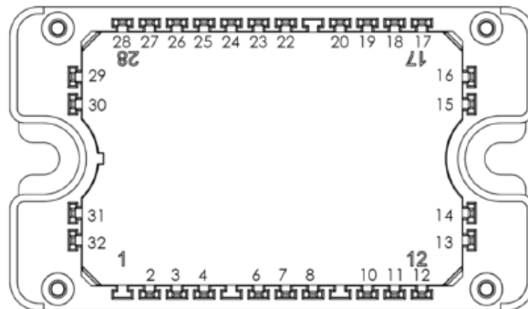
Figure 2 • MSCSM120TAM31CT3AG Pinout Location
