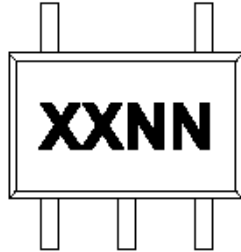
5-Lead SOT-23 (MCP6V71, MCP6V71U)
