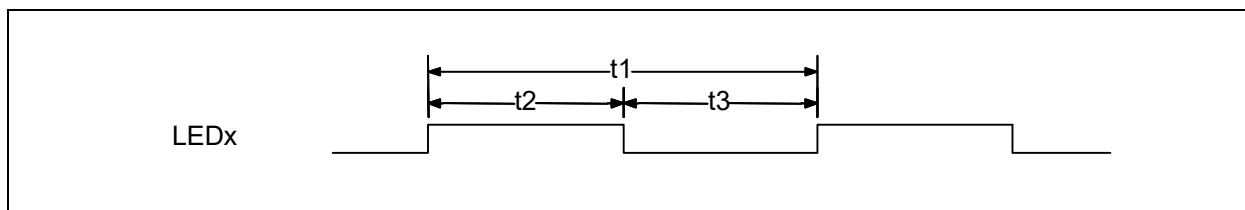
FIGURE 34-9: BLINKING/BREATHING PWM OUTPUT TIMING
